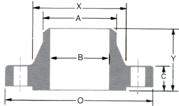
WELD NECK
