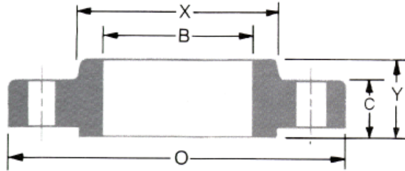
SLIP-ON
