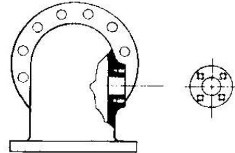
FLANGE BOSS WITH BLIND TAPPED HOLES
