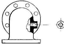
REGULAR BOSS WITH PIPE TAP
