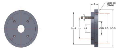
Compact Flange Reducers
