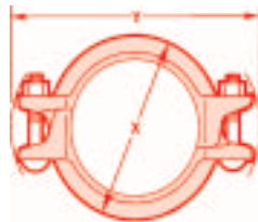
Couplings NH75
